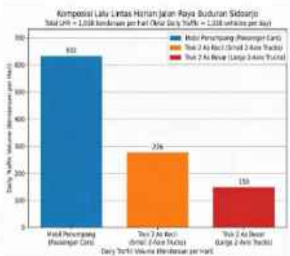
Gambar 1: Daily traffic composition on Jalan Raya Buduran showing vehicle type distribution.
